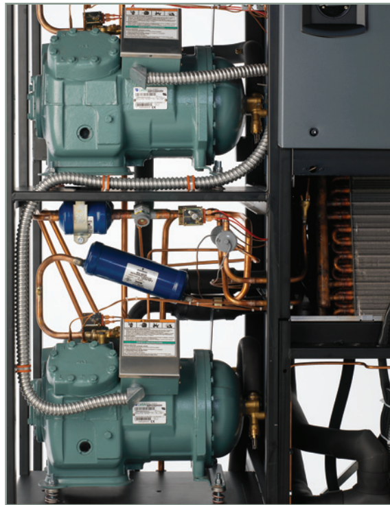
Semi-Hermetic Compressors
