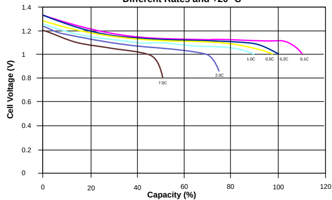
Typical Discharge curves for KFH - type Cell at Different Rates and +20° C
