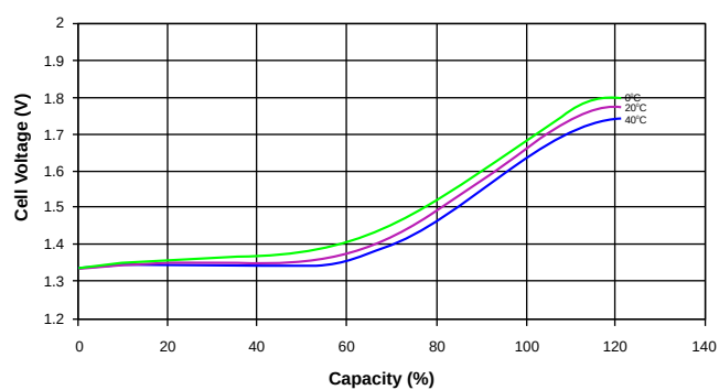
Typical charge curves for NCFP cells at constant current at 0.2C rate and different temperature
