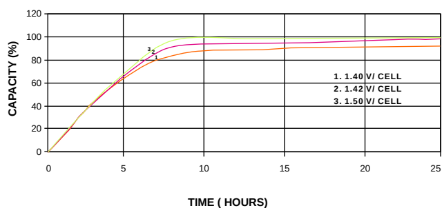
Typical charge Characteristic Of NCFP cells at Different Constant Voltages at +20°C (Current limit 0.2 C 0 )
