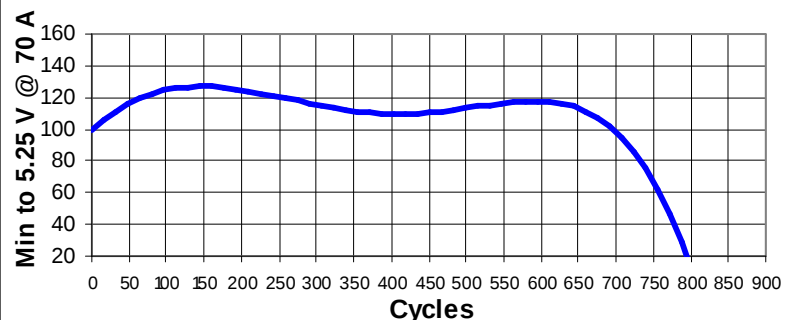
BCI- EV 2 Hour Test on Golf Car Batteries GC-15
